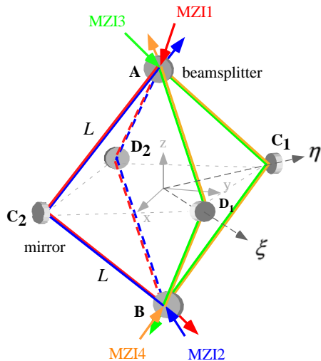
Figure 1. The 3-D DFI configuration. It consists of 4 Mach-Zehnder interferometers, MZI1, MZI2, MZI3 and MZI4. A and B are beamsplitters, and C_{1,2} and D_{1,2} are steering mirrors. Path lengths between mirrors and beamsplitters are L . The light path of MZI1 is A_t D_2 B_r - A_r C_2 B_t ; MZI2 is B_t D_2 A_r - B_r C_2 A_t ; MZI3 is A_t C_1 B_r - A_r D_1 B_t ; MZI4 is B_t C_1 A_r - B_r D_1 A_t . The subscripts r and t denote reflection and transmission at the beamsplitters.
