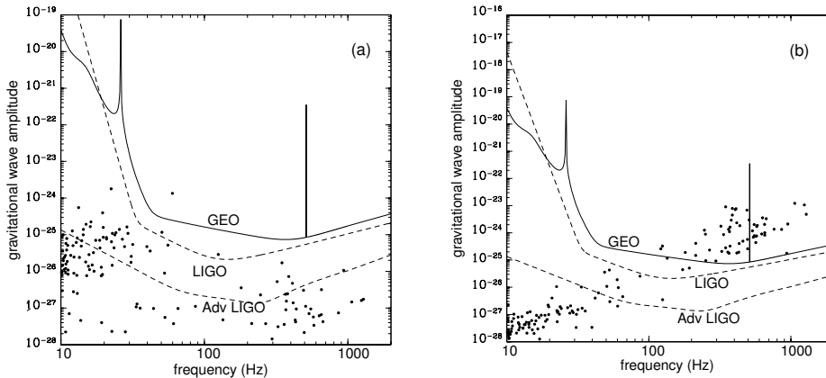
Figure 1. Theoretical strain signals from known pulsars after one year of integration, (a) attributing the rate of loss of rotational kinetic energy to gravitational luminosity and (b) assuming an equatorial ellipticity of 10^{-5} . The one-year theoretical sensitivities for GEO, LIGO and Advanced LIGO are also shown.
