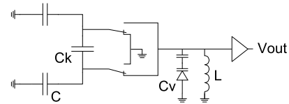
Figure 4: An amplification scheme using two relays and one tuning diode C_v .
