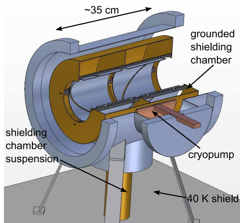
Figure 2: Preliminary mechanical design of the beam position monitor.
