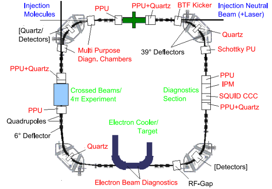
Figure 1: Overview over the CSR beam diagnostics system.
