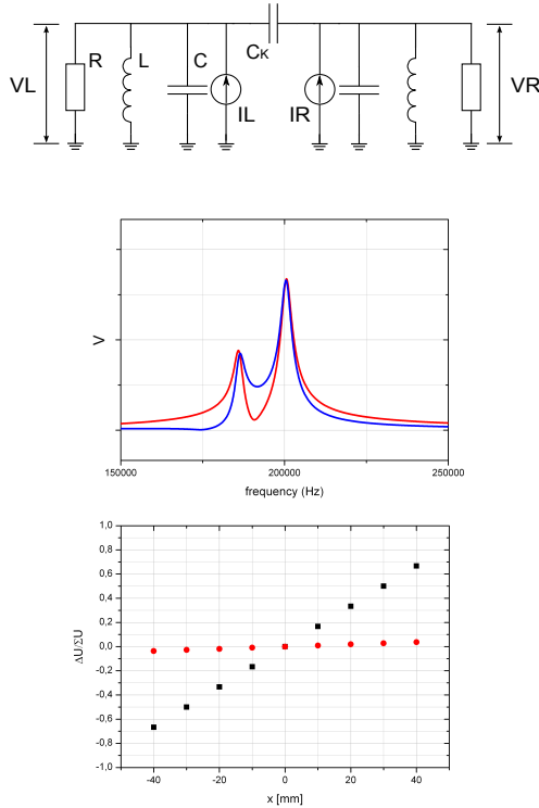
Figure 3: The effect of the coupling capacity on the resonant pickups. Upper plot: Equivalent circuit with the capacity of the pickup electrode (+cables etc.) and the coupling capacity C_k . The difference of the signal currents IL and IR is for a diagonally slit pickup linearly dependent on the beam displacement. For beam position measurements the left and right voltages VL and VR are processed. Middle: Frequency response with the resonant circuits tuned to 200 kHz and C = 4 pF. The curves (red: VR , blue: VL ) are calculated for a beam position of x = 30 mm. Lower: Plot of the calibration curves. Black: Calibration curve for non-resonant amplification, i.e. without the inductances. The slope is decreased due to coupling with respect to the ideal case where (VR - VL)/(VR + VL) = 1 at x = 50 mm. Red: Calibration curve with resonant amplification. Its slope is decreased by a factor of 20 with respect to non-resonant amplification.
